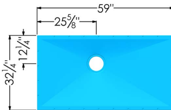
59" x 32 1/4" (Perimeter 7/8" thick)
