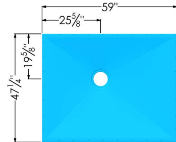
59" x 47 1/4" (Perimeter 7/8" thick)
