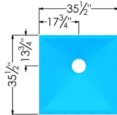
35 1/2" x 35 1/2" (Perimeter 7/8" thick)
