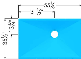
55 1/8" x 35 1/2" (Perimeter 7/8" thick)
