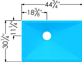
44 3/4" x 30 1/4" (Perimeter 7/8" thick)
