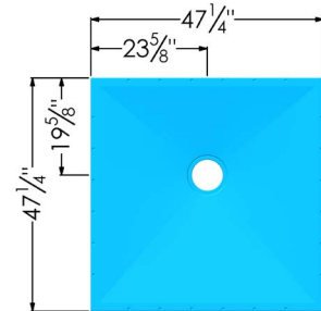
47 1/4" x 47 1/4" (Perimeter 7/8" thick)
