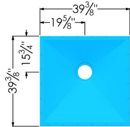
39 3/8" x 39 3/8" (Perimeter 7/8" thick)
