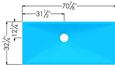
70 7/8" x 32 1/4" (Perimeter 7/8" thick)
