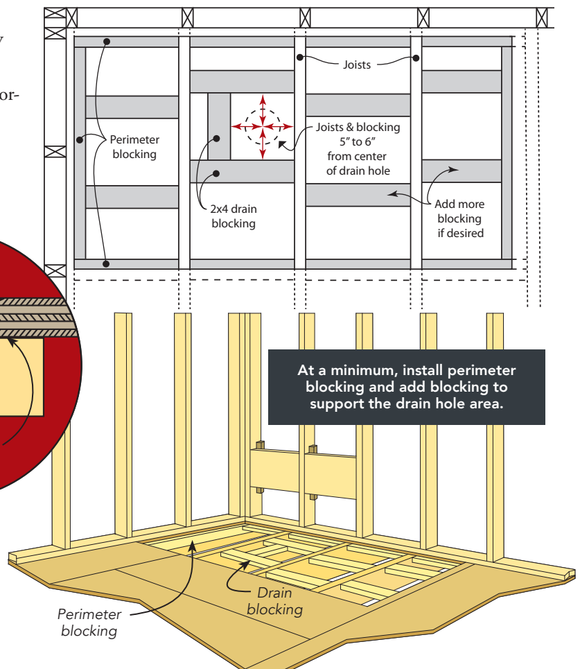
Perimeter Detail
